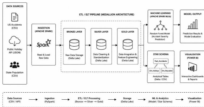
Figure 5.3: Architecture Diagram
